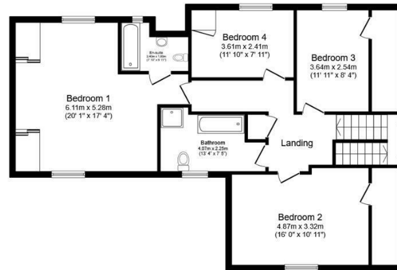
First Floor Floor area 94.3 sq.m. (1,015 sq.ft.)
